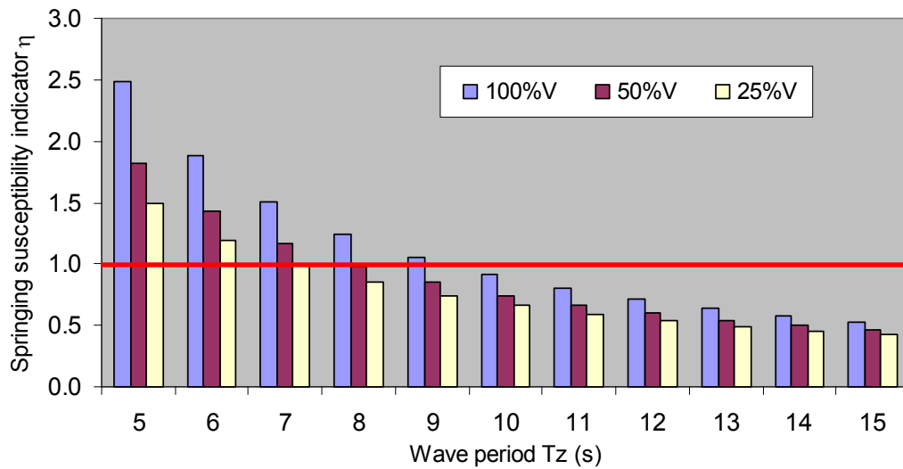
FIGURE 3 Springing Susceptibility Indicator
