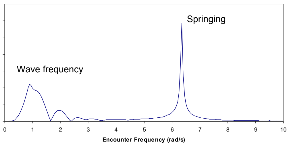
FIGURE 5 Vertical Bending RAO Distribution
