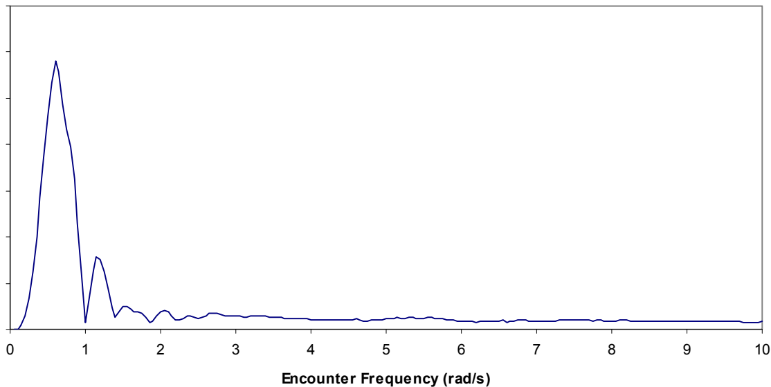
FIGURE 2 Vertical Bending Moment RAO (rigid body)
